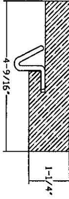
4 6 POLYURETHANE HEAD & SIDE JAMB
