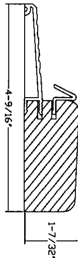
2 OUT-SWING SILL
