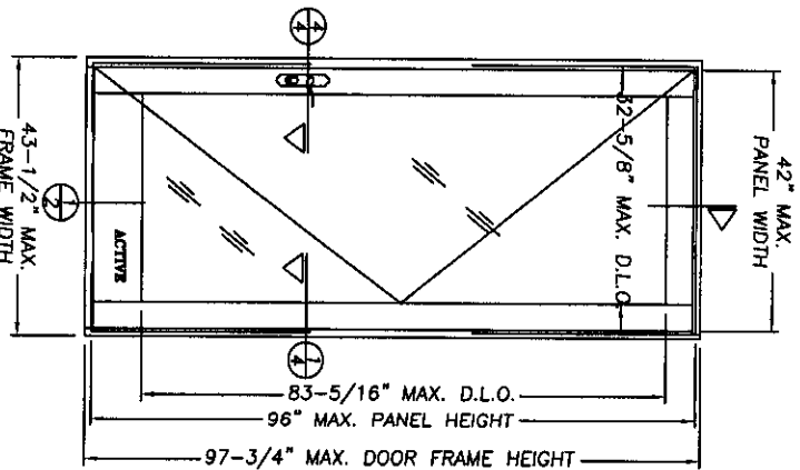
SINGLE OUTSWING UNIT
