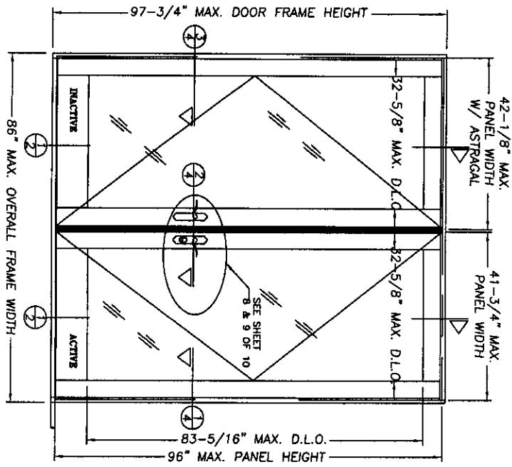
DOUBLE OUTSWING UNIT
